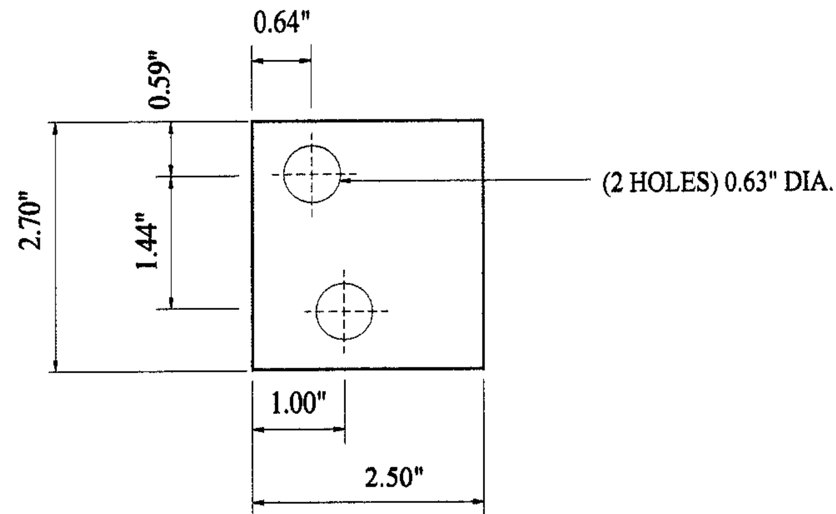
LEFT SPADE (VIEWED FROM THE BOTTOM)
