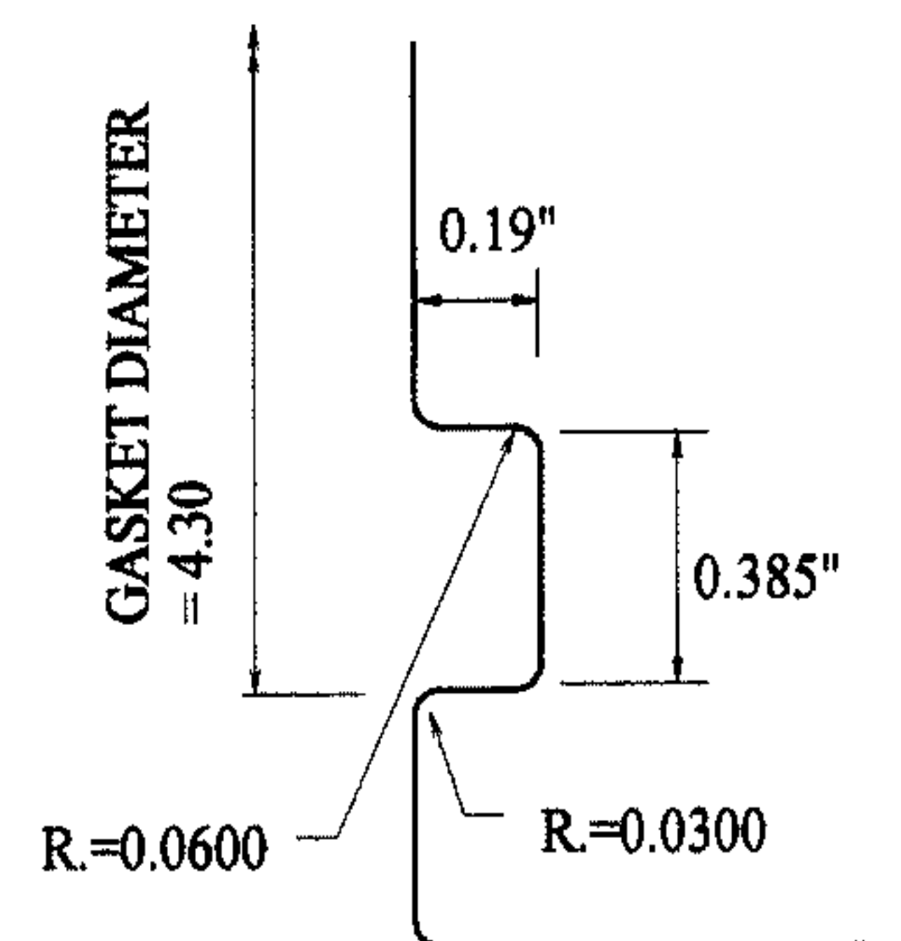
GASKET GROOVE DETAIL
