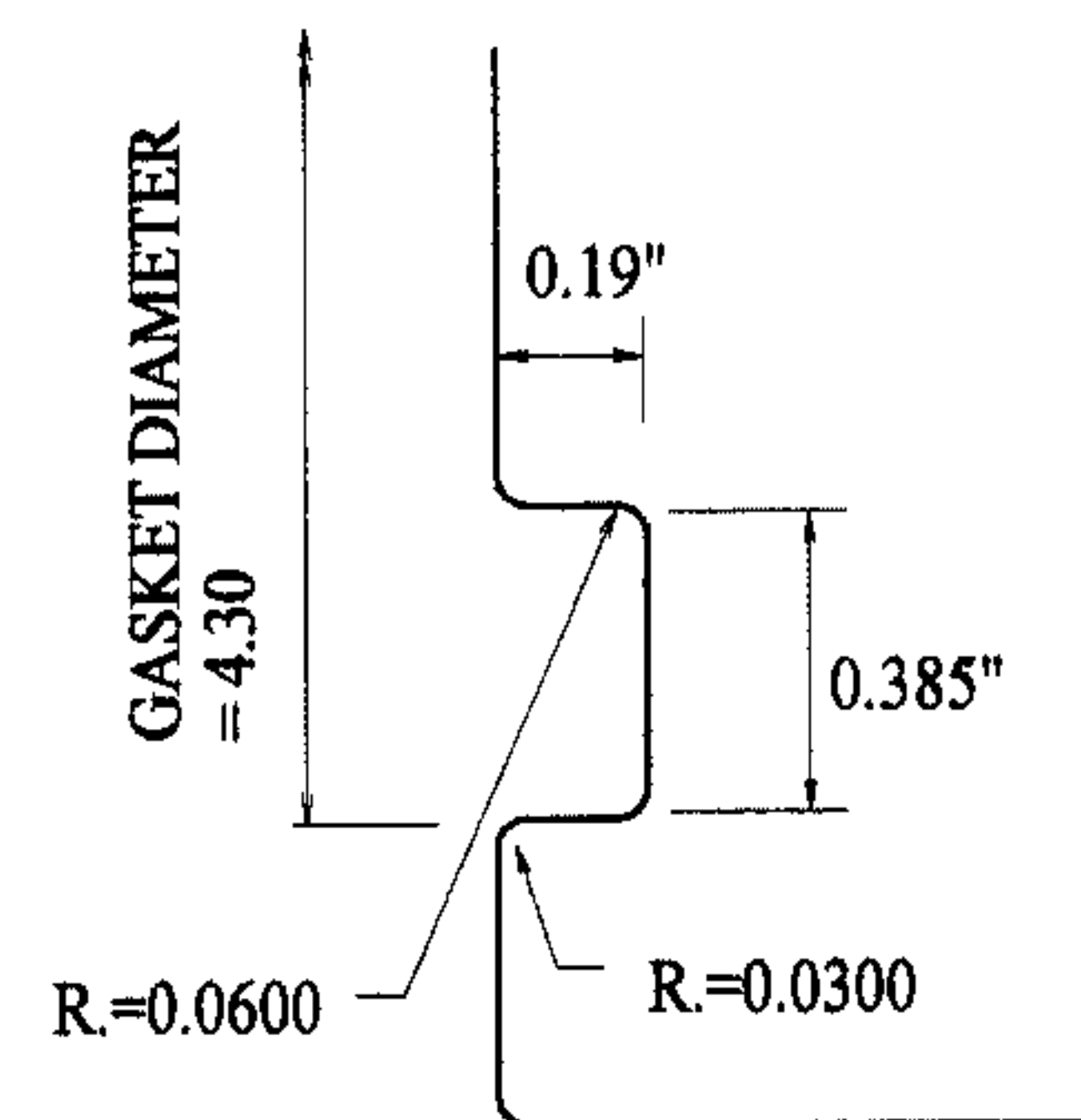
GASKET GROOVE DETAIL
