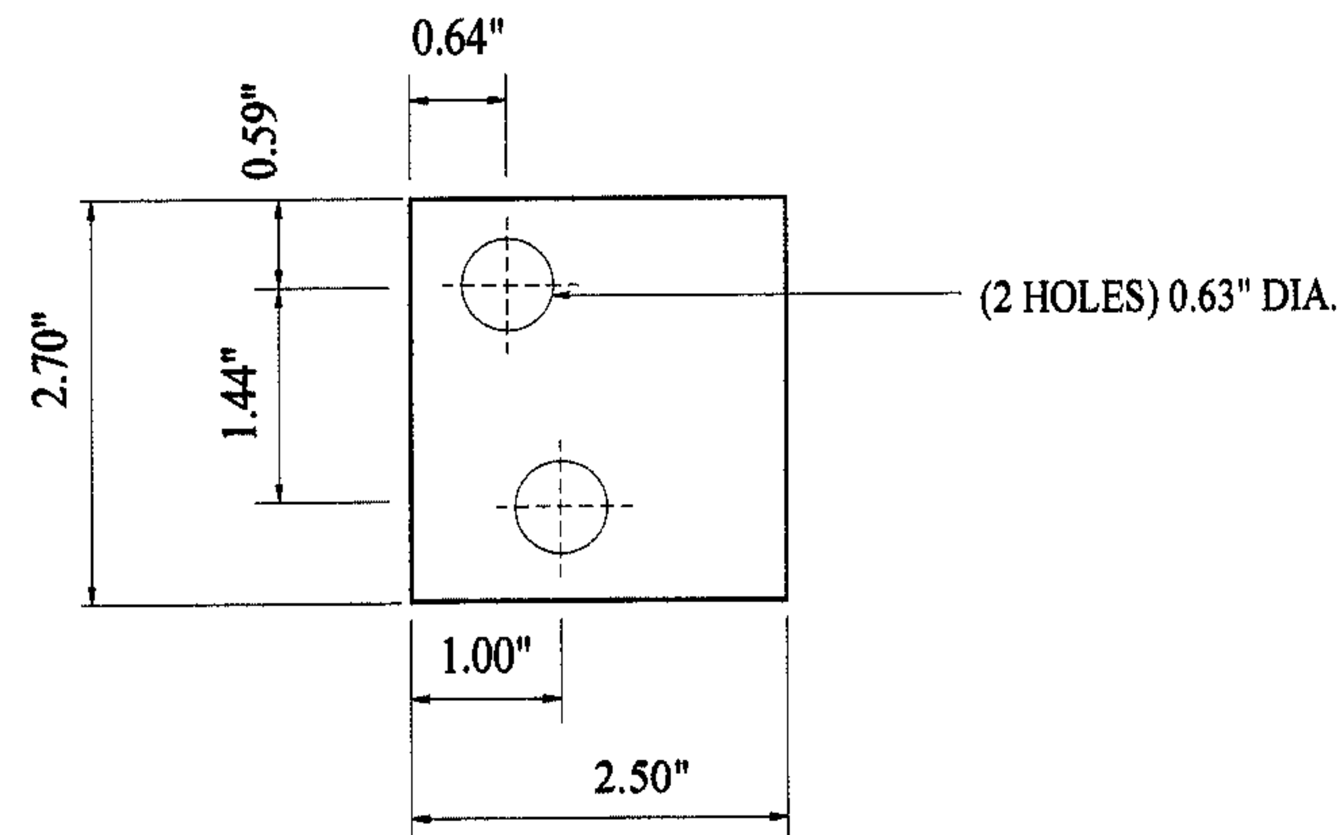
LEFT SPADE (VIEWED FROM THE BOTTOM)
