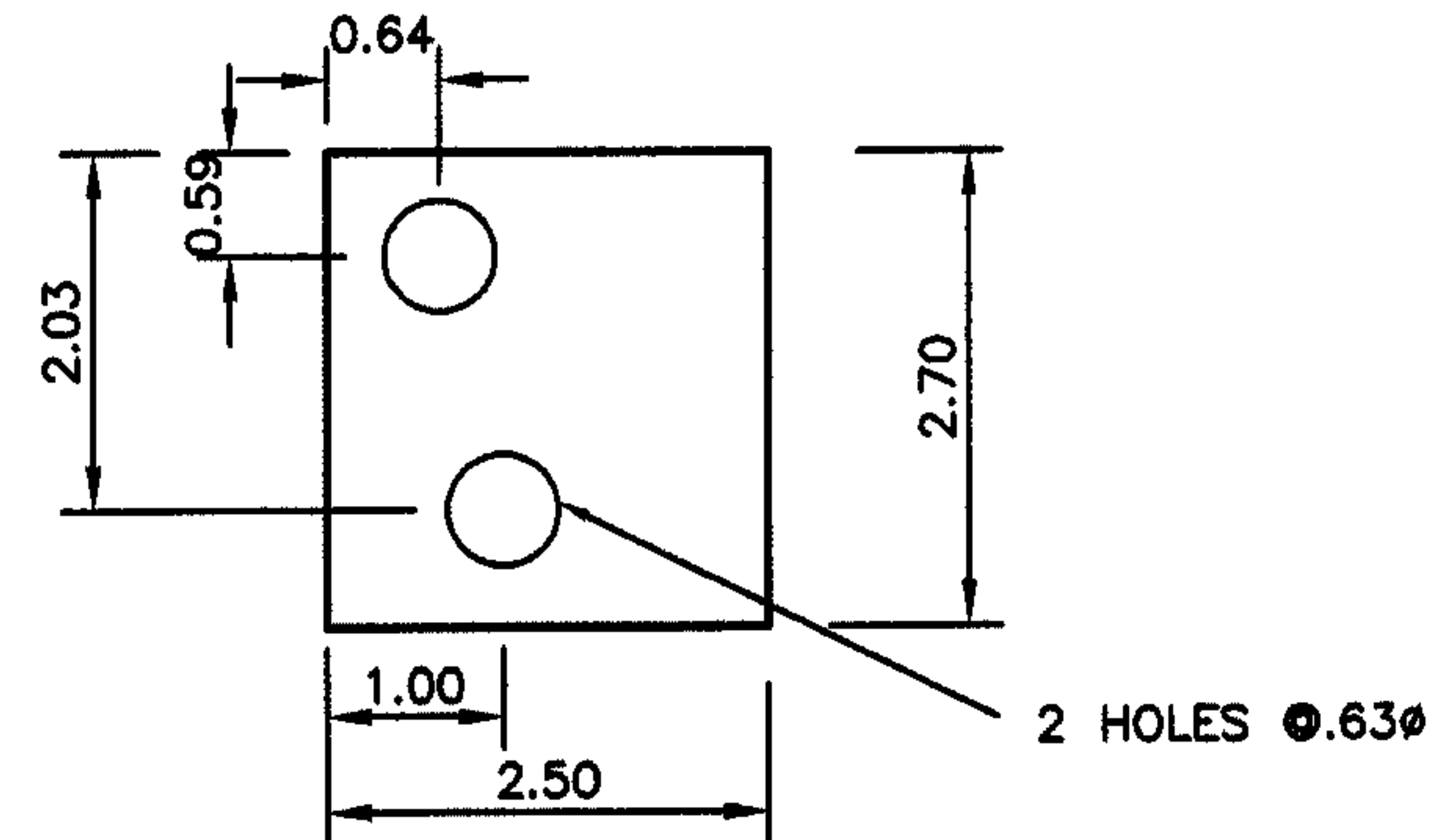
LEFT SPADE (VIEWED FROM THE BOTTOM)
