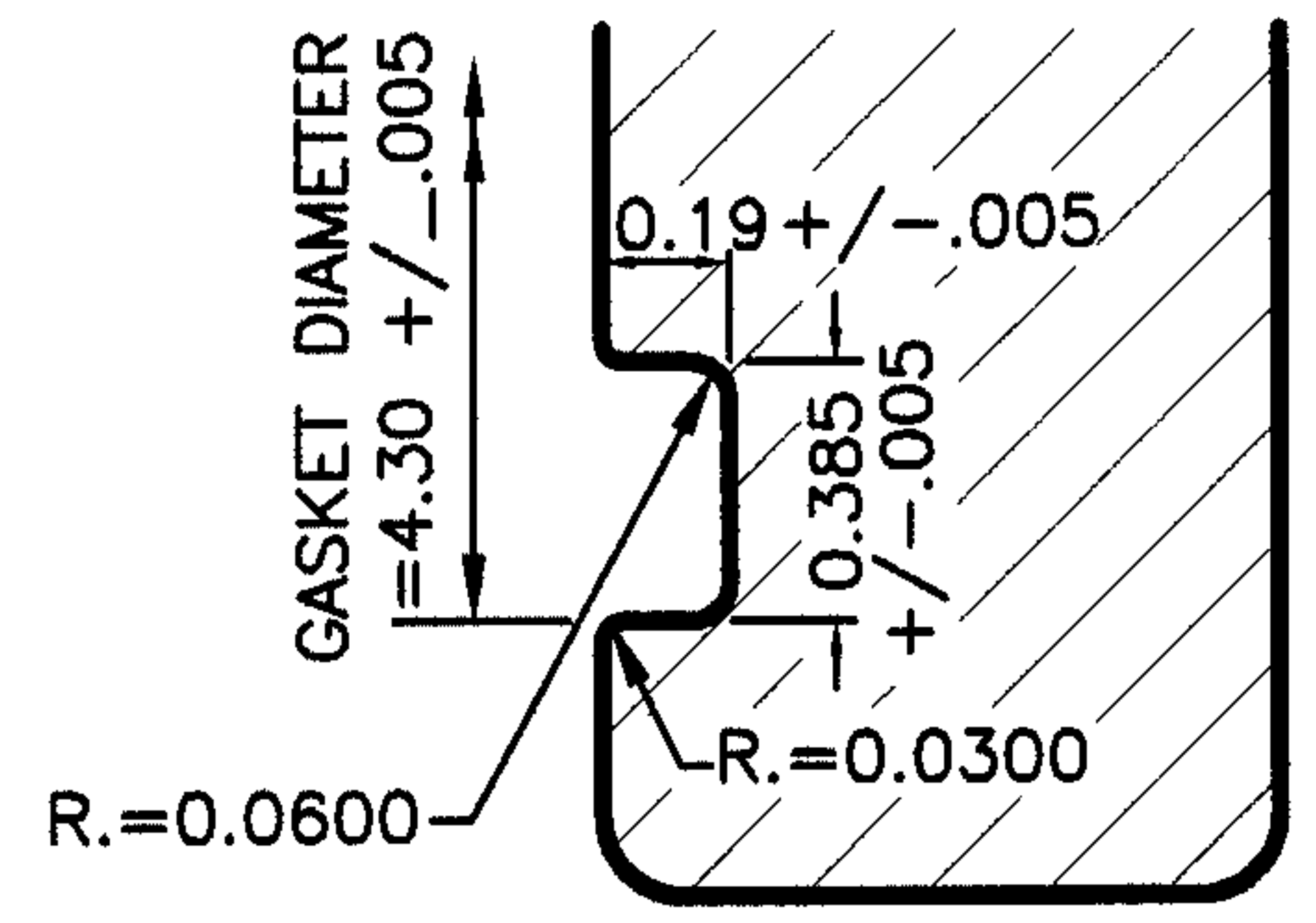
GASKET GROOVE DETAIL
